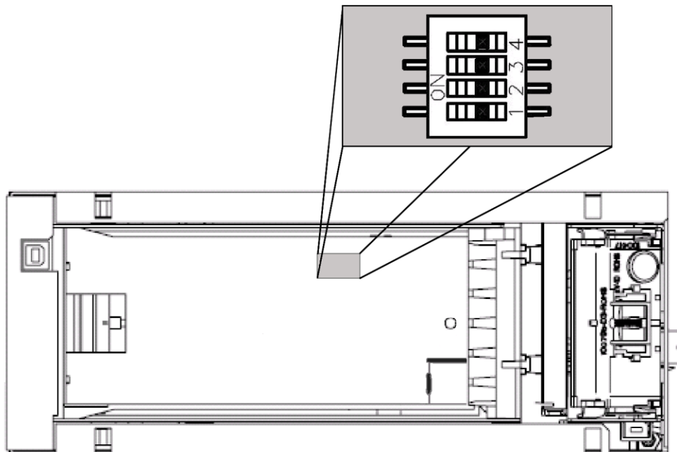
Figure 5: DIP Switch
