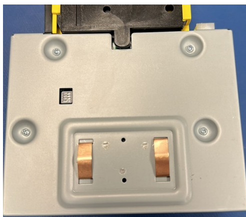
Figure 30: Base Plate
