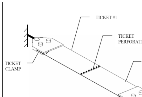
Figure 19: Perforation Test
