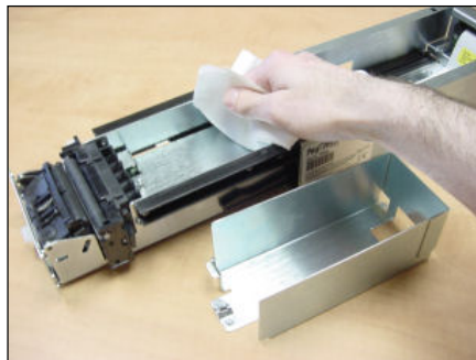
Figure 37: Remove excess dust
