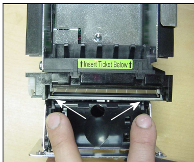
Figure 43: Bottom paper guide inspection
