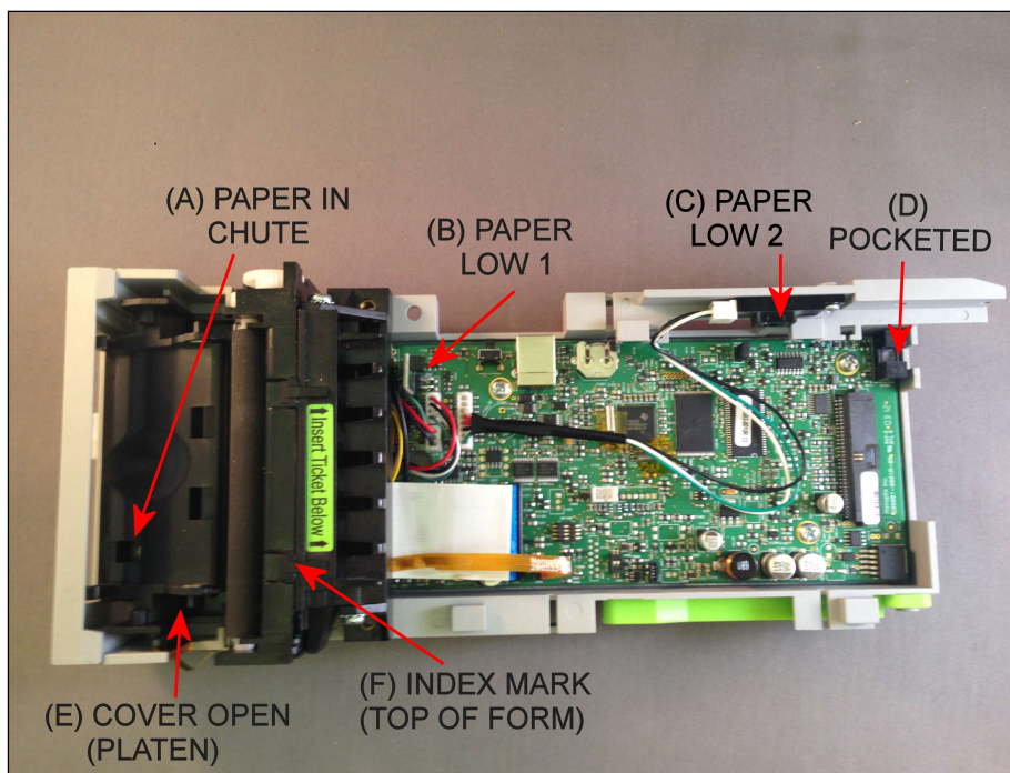
Figure 17: Sensors
