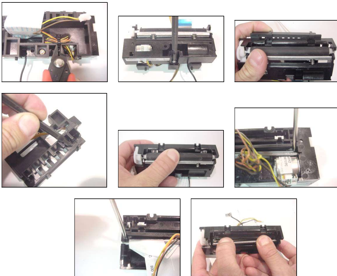
Figure 35: Disassembly
