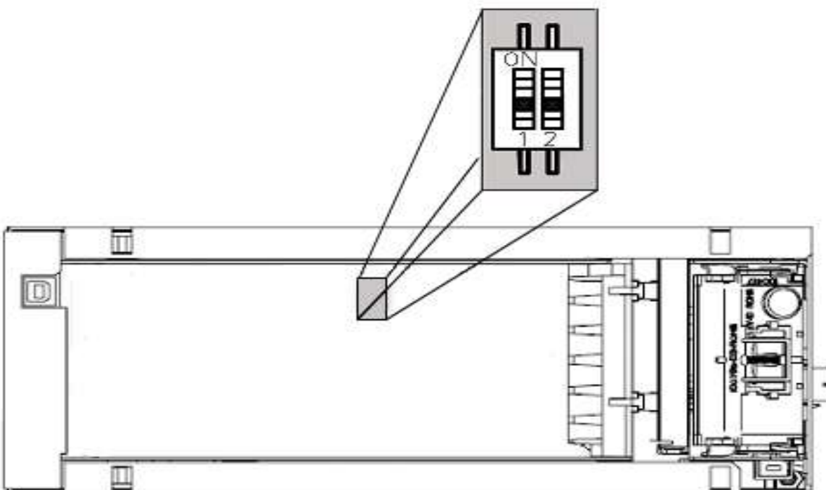
Figure 9: Boot Selector
