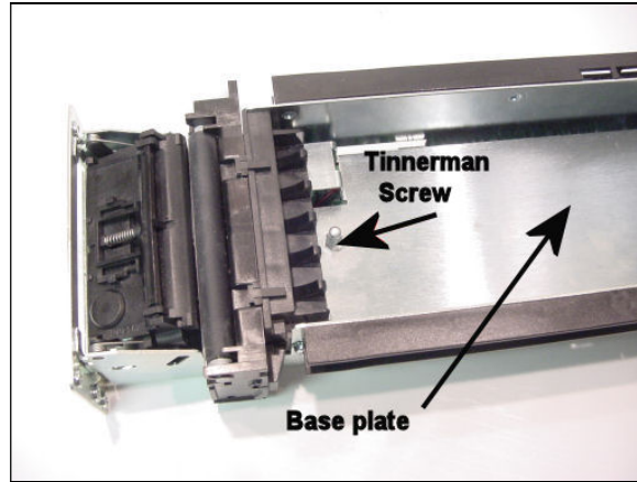
Figure 24: Base Plate
