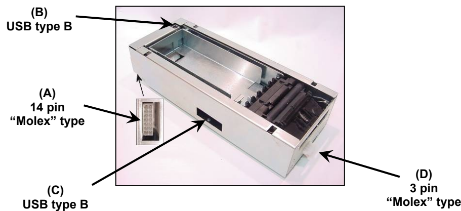
Figure 5: Interface Ports
