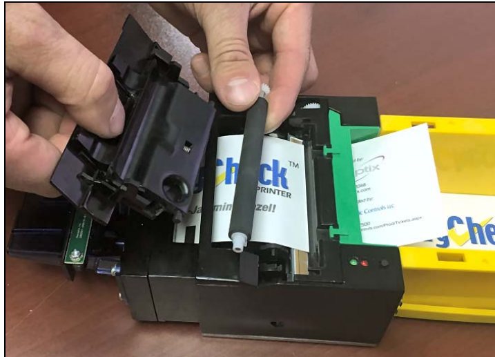
Figure 17: Clearing Jams
