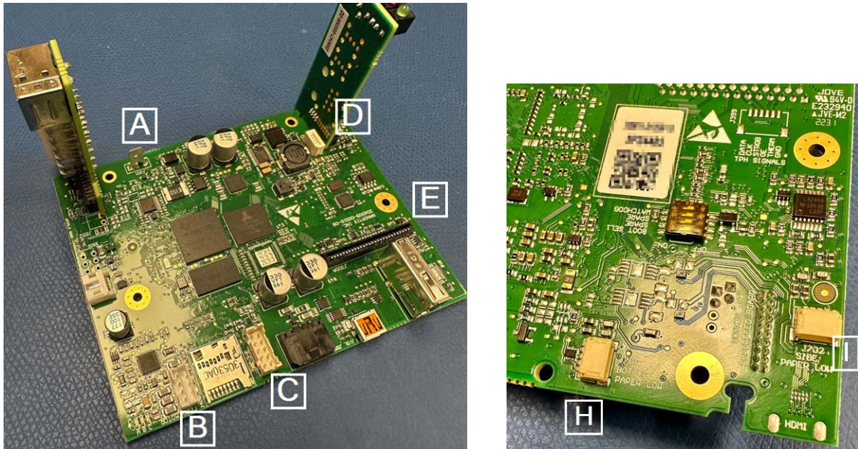
Figure 19: Connector Layout (Rev 2 shown)
