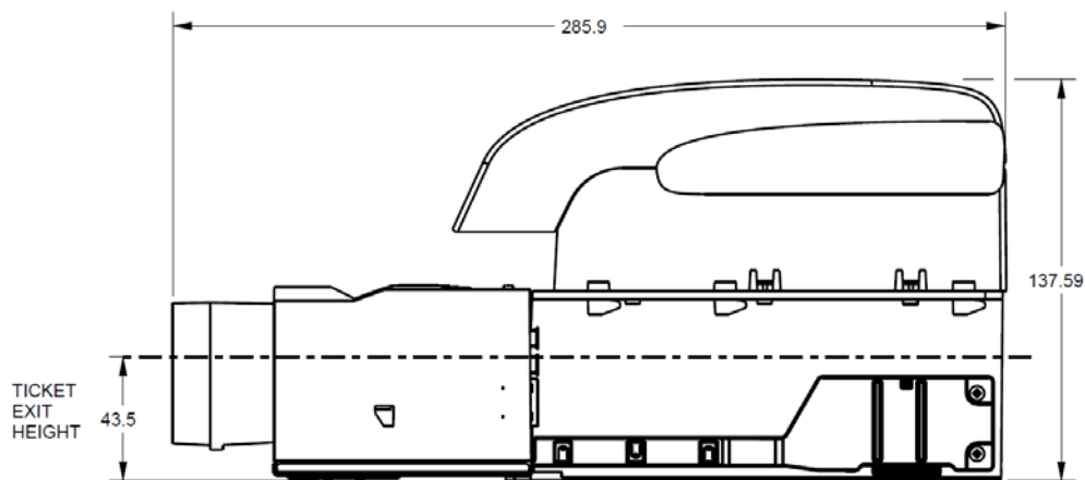
Figure 28: Dimensions – Right side (800 ticket extension)
