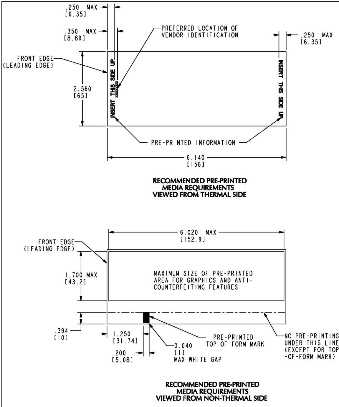
Figure 21: Ticket Specifications
