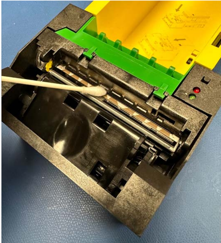
Figure 46: Clean heating elements
