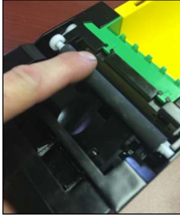
Figure 43: Remove Roller
