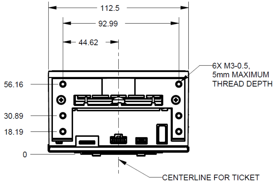
Figure 24: Dimensions - Front
