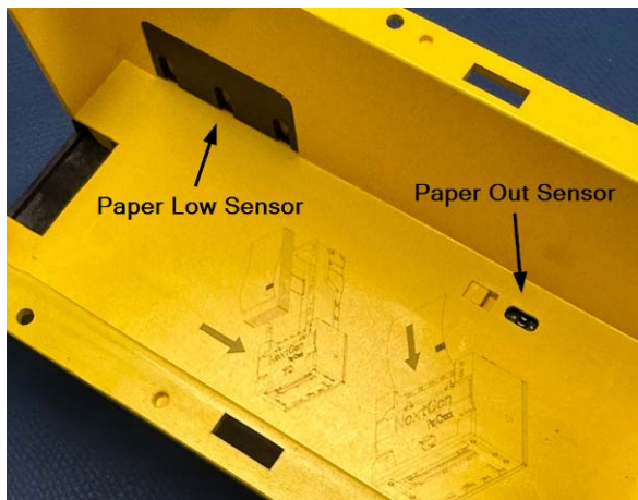
Figure 14: Paper low
