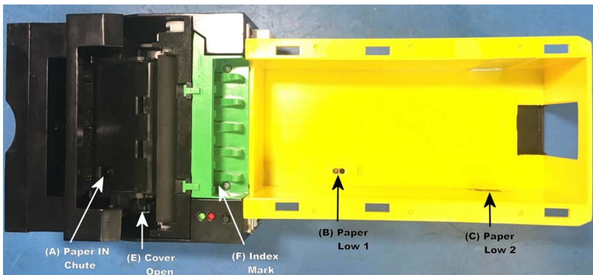
Figure 18: Sensors
