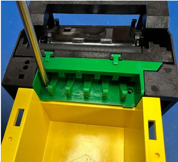
Figure 33: Ticket Inlet & Index sensor
