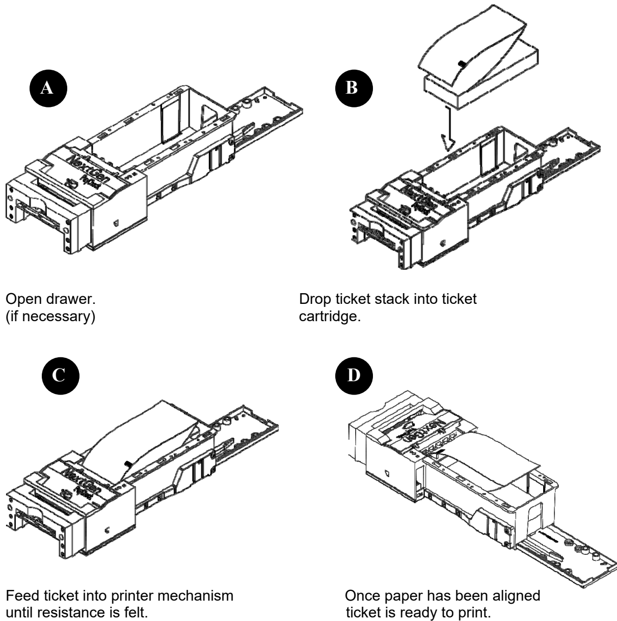
Figure 5: Loading Paper
