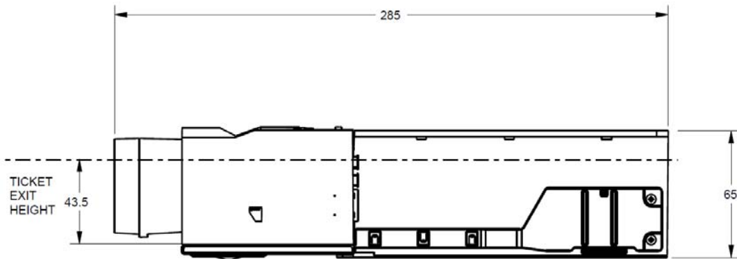
Figure 26: Dimensions – Right side (no ticket extension)
