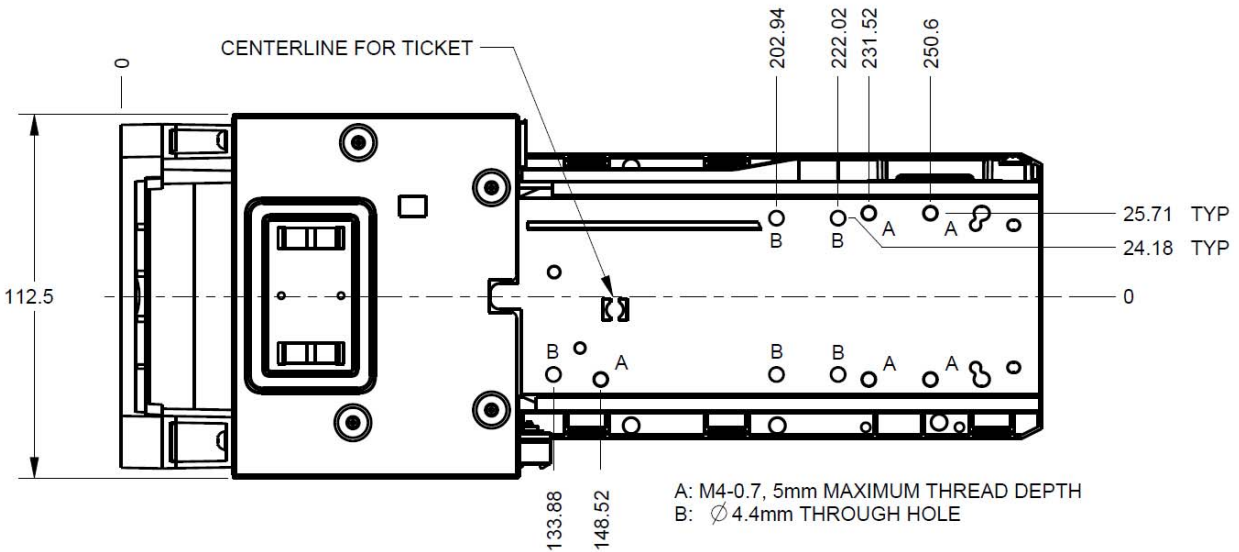
Figure 25: Dimensions - Bottom
