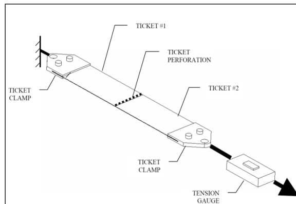
Figure 20: Perforation Test
