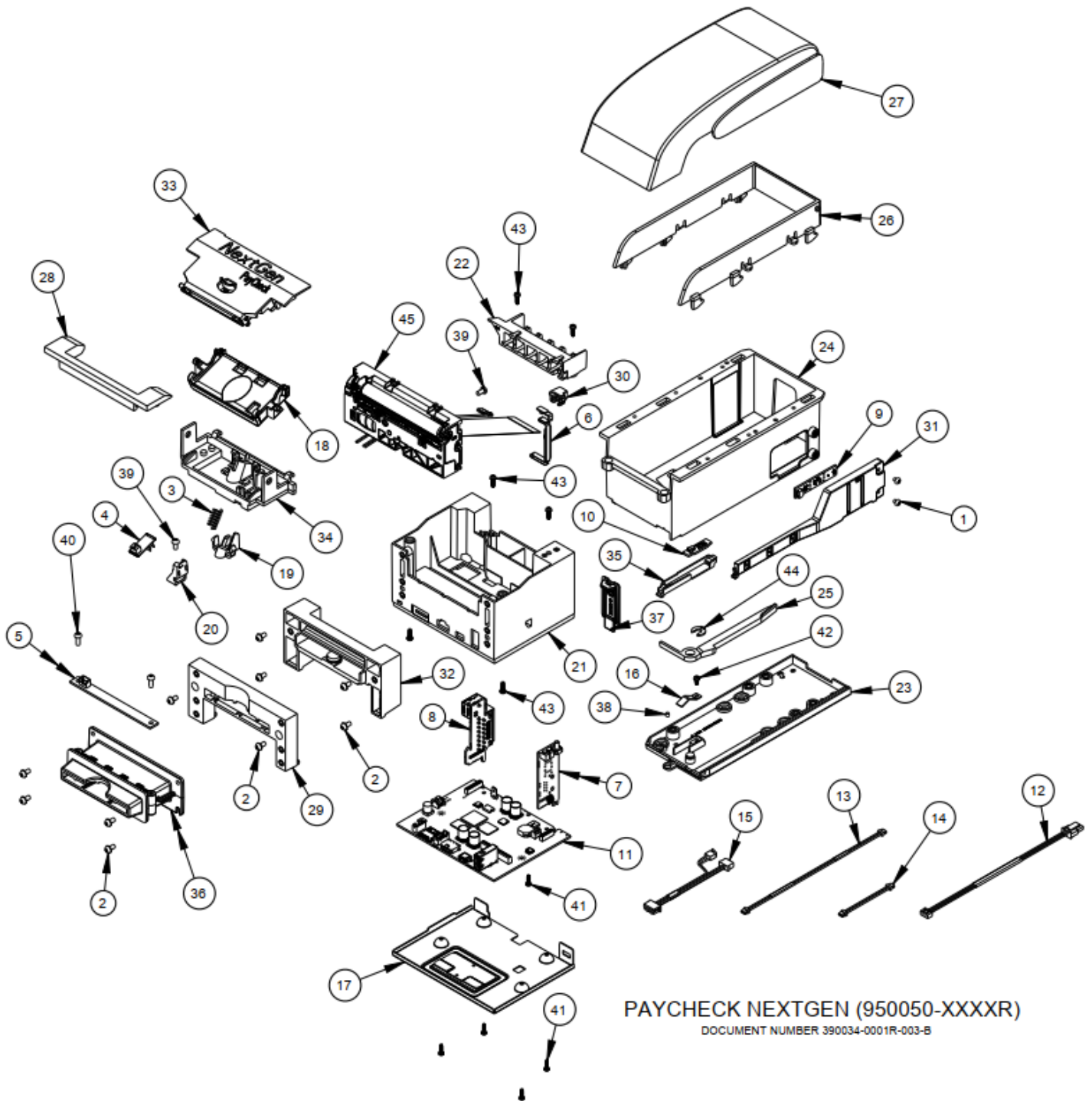
Figure 23: Exploded View
