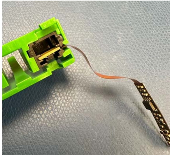
Figure 33: Ticket Inlet & Index sensor
