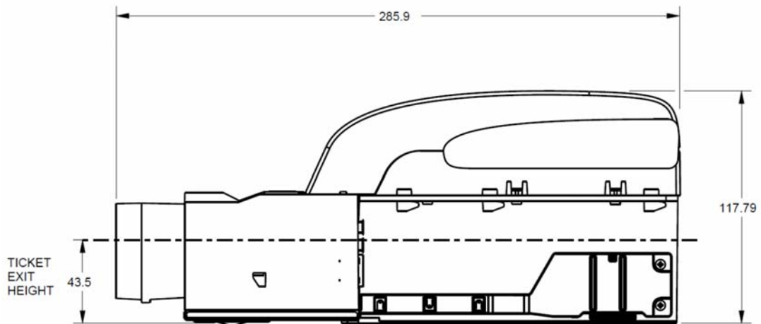
Figure 27: Dimensions – Right side (600 ticket extension)
