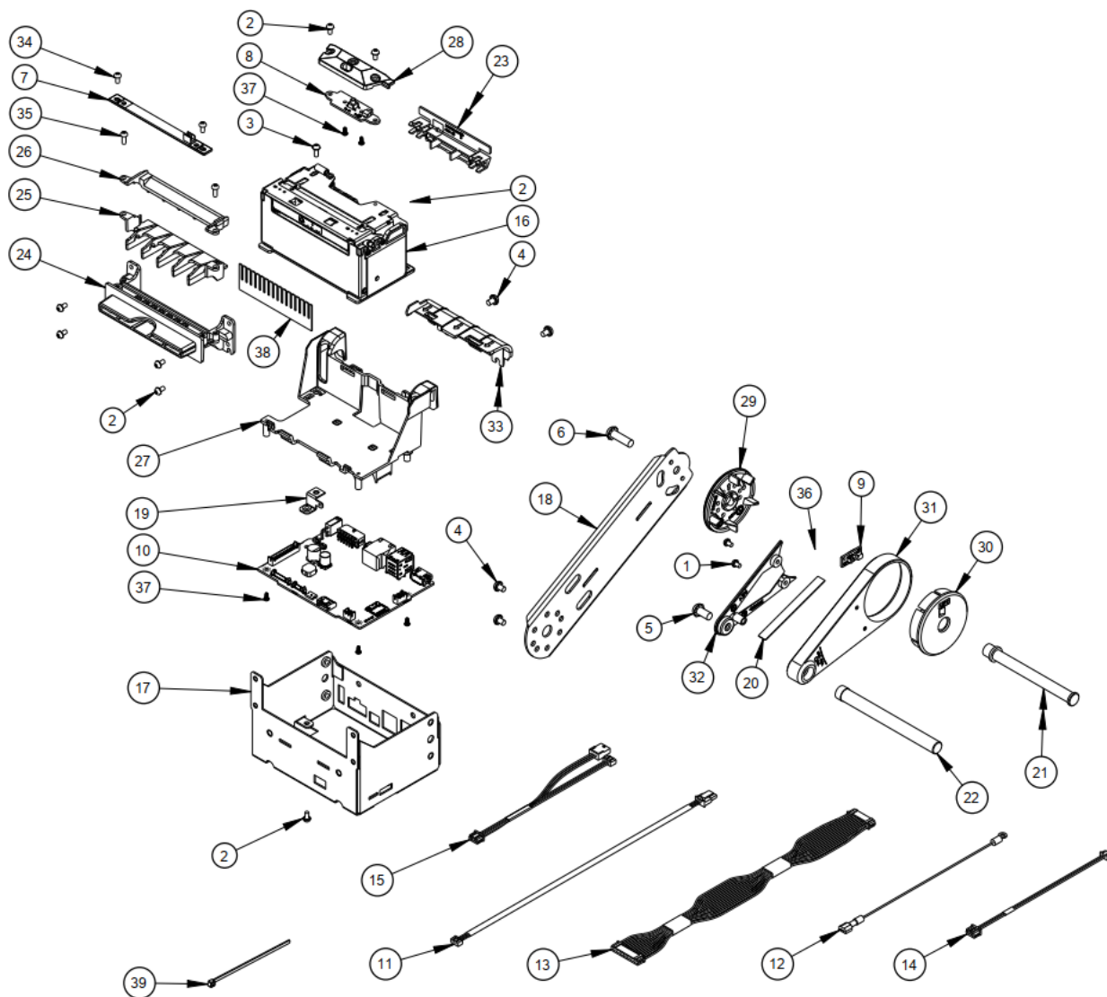
Figure 8: Exploded View
